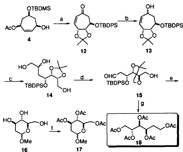
Scheme 3. (a) i. TPSCl, imidazole, DMF; ii. OsO 4 , N -methylmorpholine N -oxide, THF-H 2 O; iii. 2,2-dimethoxypropane, TsOH; iv. 0.05 N KOH, MeOH; v. MsCl, Et 3 N, CH 2 Cl 2 ; vi. pyridinium tosylate, MeOH; vii. PDC, CH 2 Cl 2 ; (b) DIBAL-H, Et 2 O; (c) i. O 3 , -78 °C, Me 2 S; ii. NaBH 4 , MeOH; (d) NaIO 4 /SiO 2 , CH 2 Cl 2 ; (e) i. Dowex-50 (H + ), MeOH; ii. Bu 4 NF-THF; (f) Ac 2 O-pyridine; (g) i. 6 N HCl, THF, ii. Ac 2 O-pyridine.
