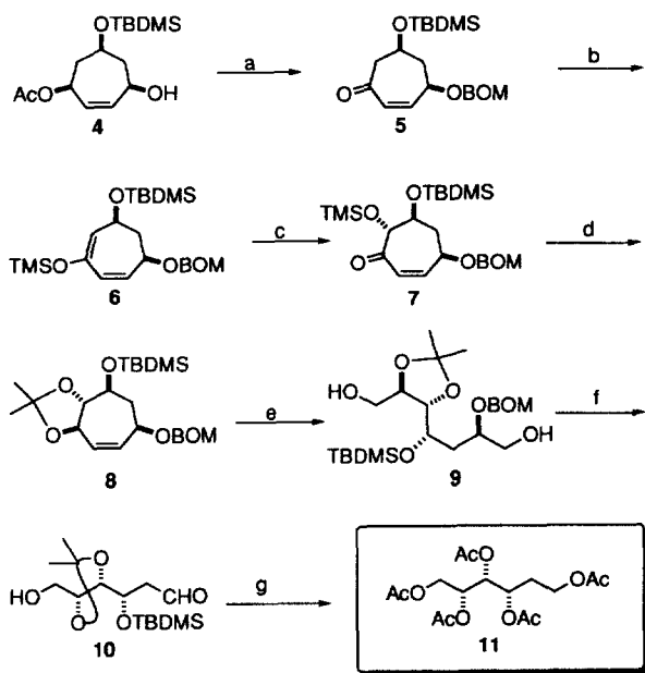
Scheme 2. (a) i. BOMCl, 2-Pr 2 EtN, CH 2 Cl 2 ; ii. 0.05 N KOH, MeOH; iii. PDC, CH 2 Cl 2 ; (b) TMSOTf, Et 3 N; (c) m -CPBA, CH 2 Cl 2 ; (d) i. DIBAL-H, Et 2 O, -78 °C; ii. 2,2-dimethoxypropane, TsOH; (e) i. O 3 , CH 2 Cl 2 , -78 °C, Me 2 S; ii. NaBH 4 , MeOH; (f) i. H 2 , Pd/C, AcOEt; ii. NaIO 4 /SiO 2 , CH 2 Cl 2 ; (g) i. NaBH 4 , MeOH; ii. HCl (aq), MeOH; iii. Ac 2 O-pyridine.
